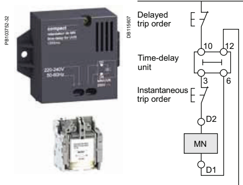
PE103752-32 DB115607 MN release with a time-delay unit.
