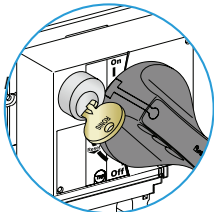
Rotary-handle locking using a keylock.
