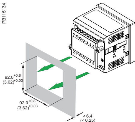
EM6400NG multi-function meter flush mounting type
